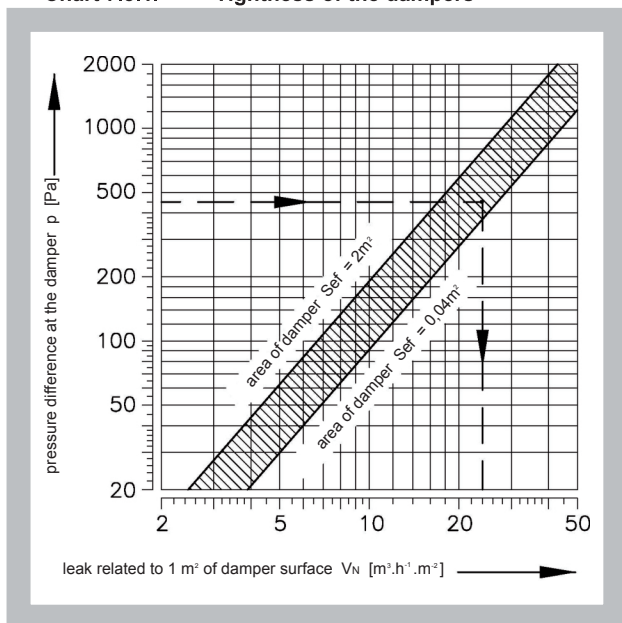
Chart 7.3.1. Tightness of the dampers
