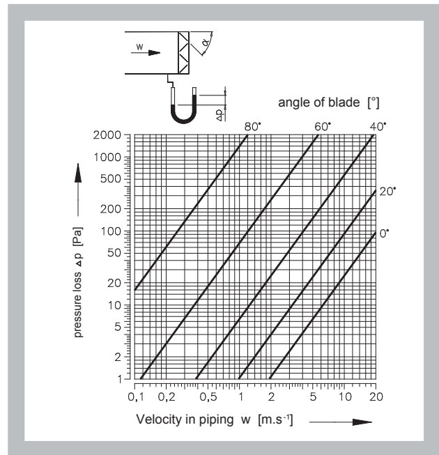
Chart 7.2.2. Regulation damper attached to the end of the duct
