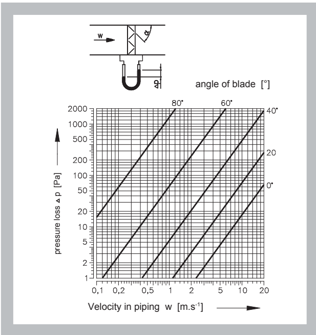
Chart 7.2.1. Regulation damper inserted into the duct
