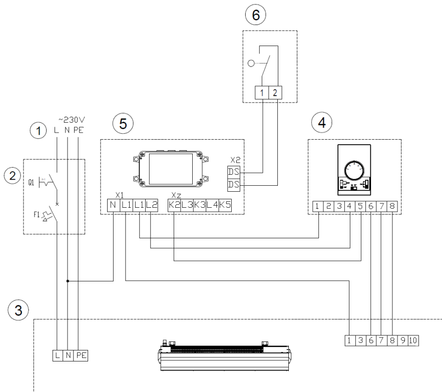
Figure 1 – W100 AC, W150 AC, W200 AC connections
