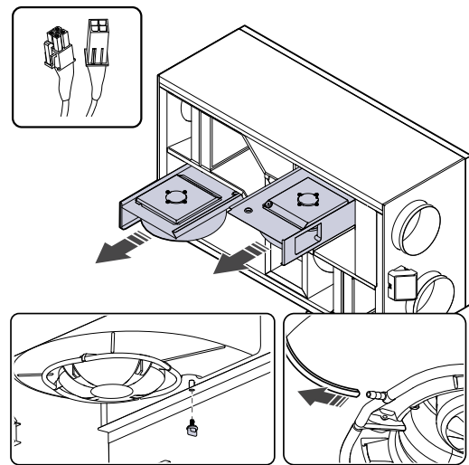
Fig. 3 Extract and supply air fans
