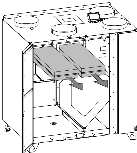
Fig. 4 Changing of filters
