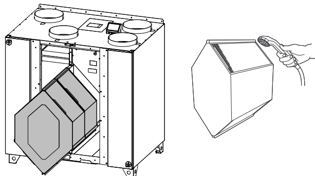
Fig. 5 Removing and cleaning the heat exchanger
