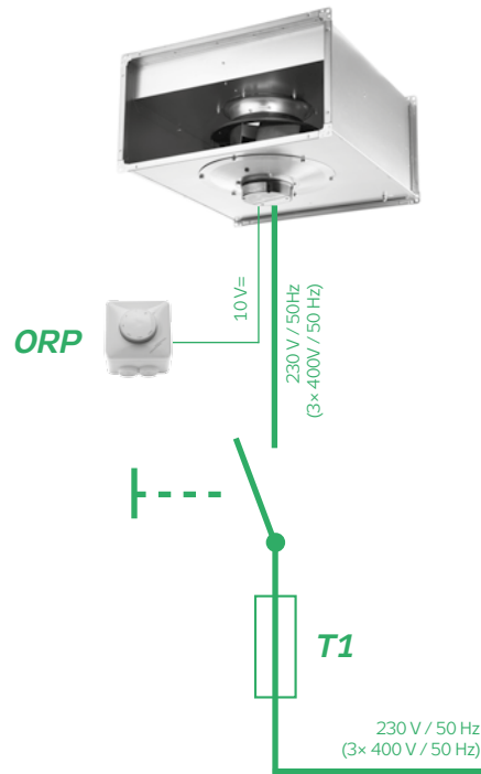
FIGURE 7 – FAN CONNECTION
