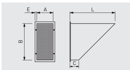
ASV KABT Protection guards Wire protection guards for mounting on the cabinet fan discharge.
